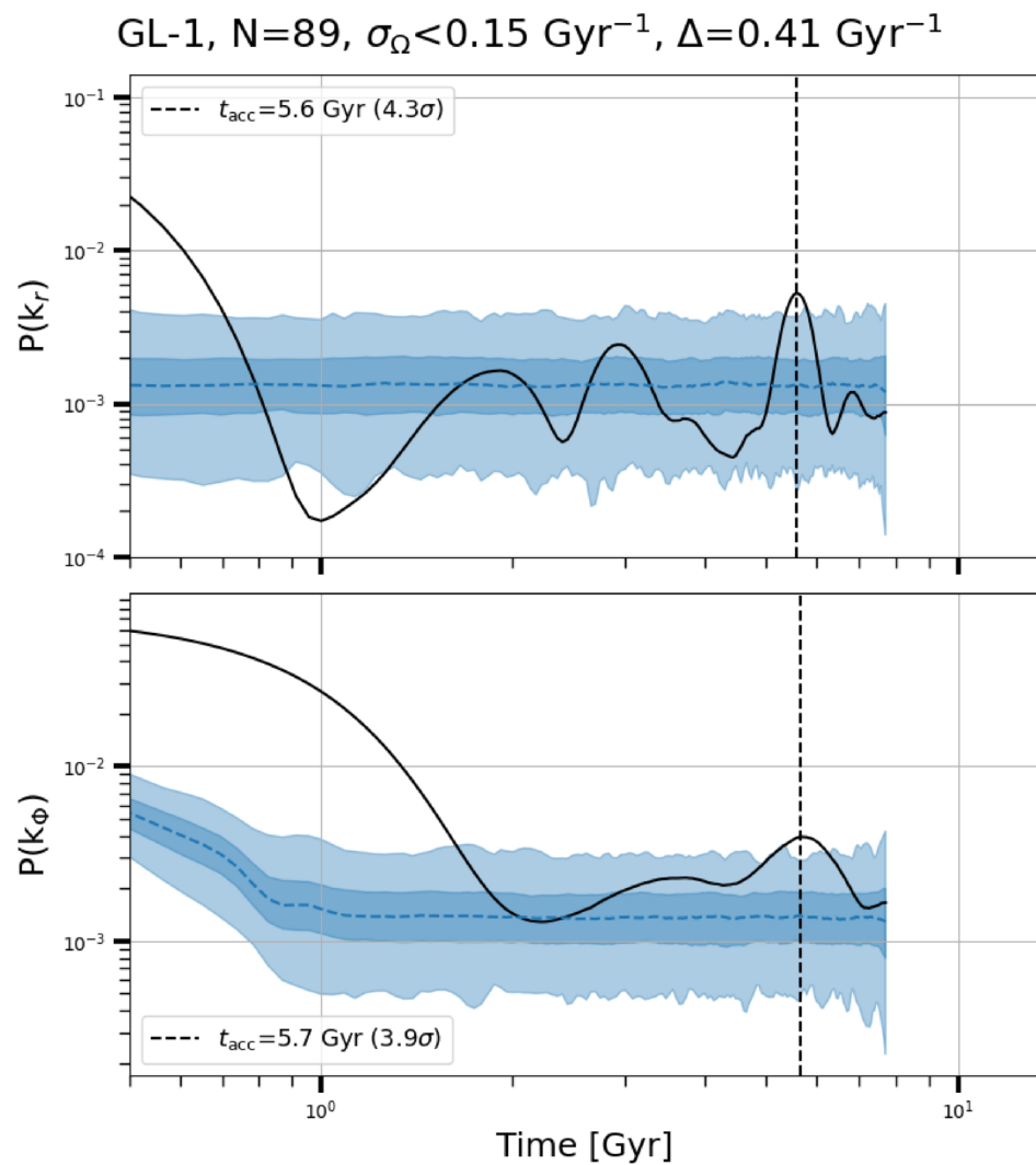
Figure 5. from Hefan Li et al 2026 Astron. J. 171 doi:10.3847/1538-3881/ae3a83 https://dx.doi.org/10.3847/1538-3881/ae3a83 © 2026. The Author(s). Published by the American Astronomical Society.
