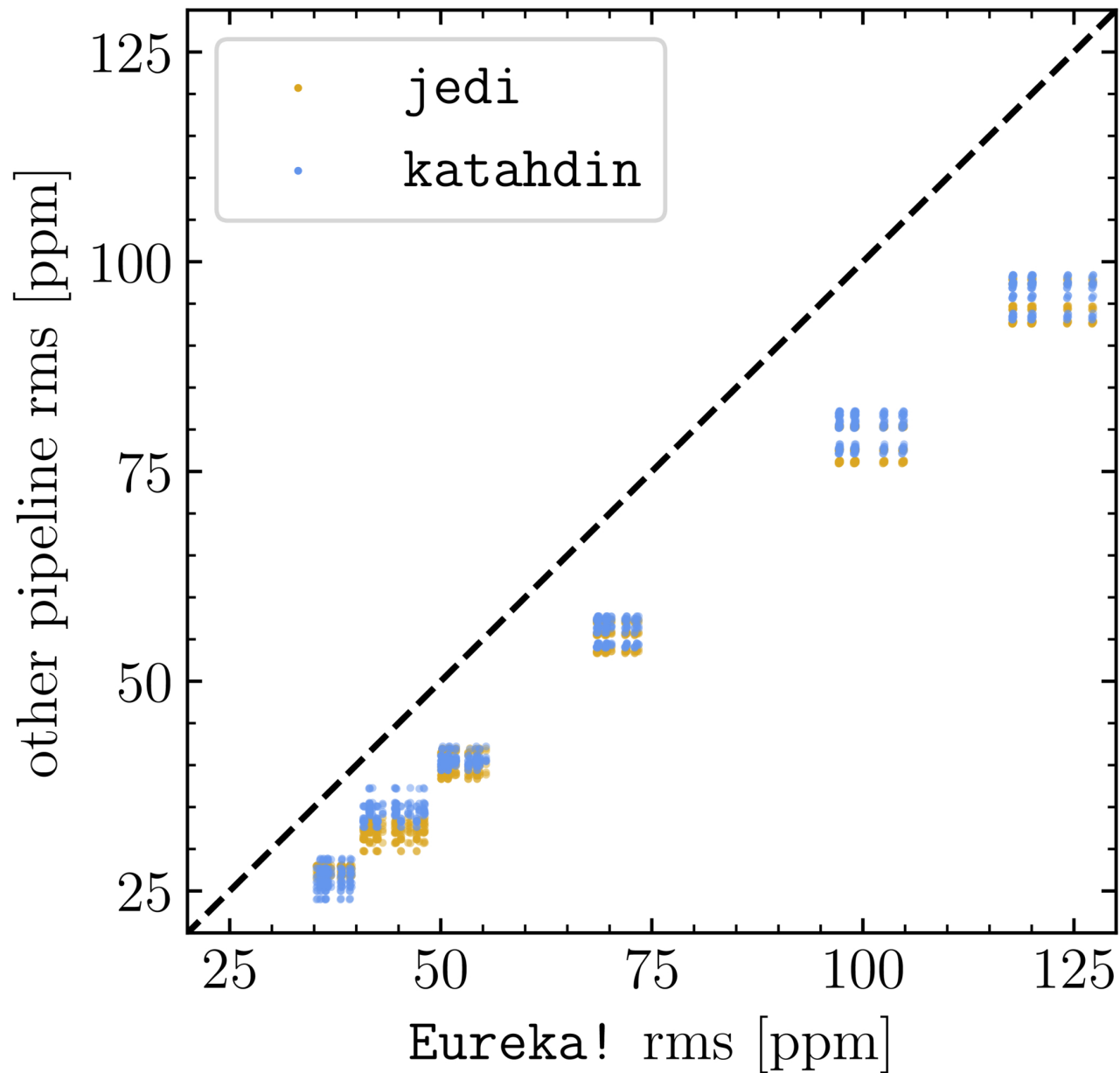
Figure 9. from Ben Cassese et al 2026 Astron. J. 171 doi:10.3847/1538-3881/ae3a81 https://dx.doi.org/10.3847/1538-3881/ae3a81 © 2026. The Author(s). Published by the American Astronomical Society.
