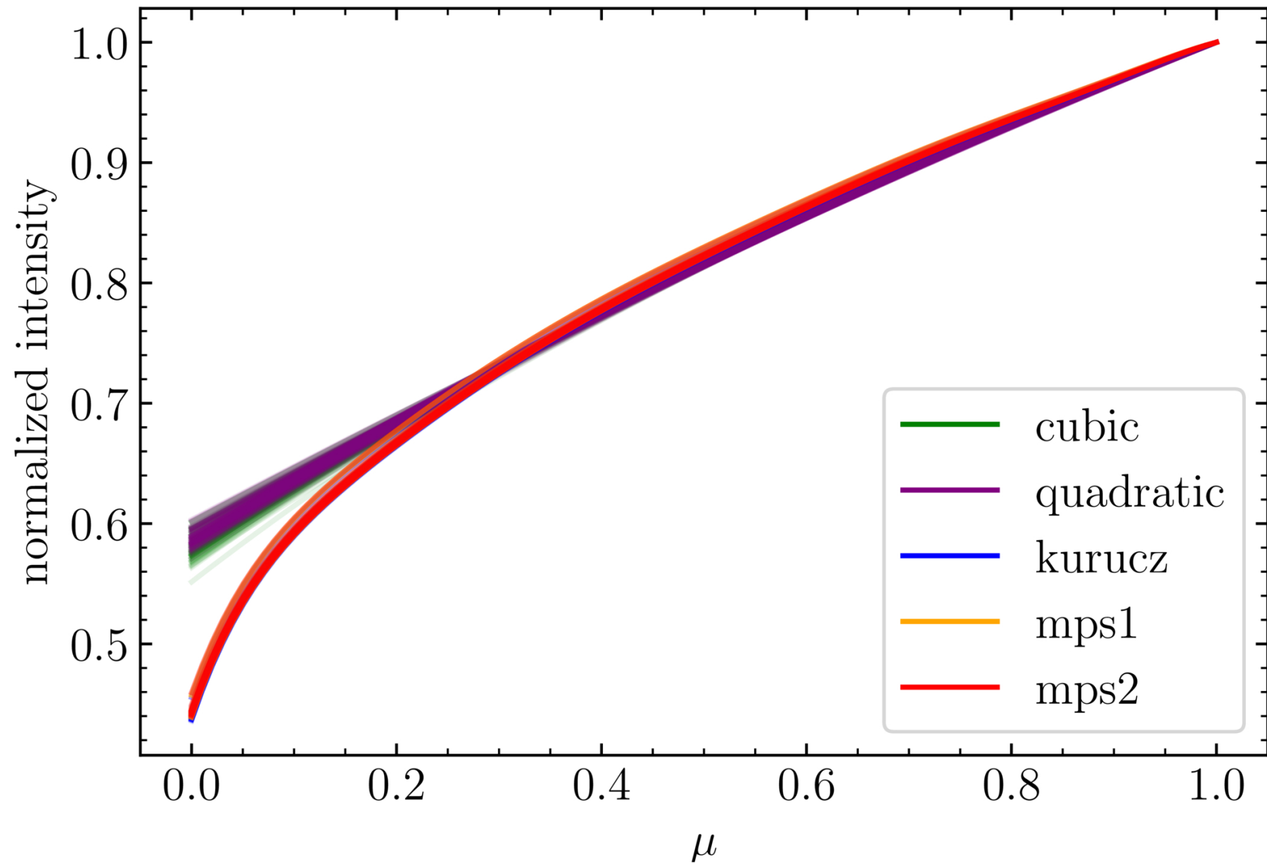
Figure 8. from Ben Cassese et al 2026 Astron. J. 171 doi:10.3847/1538-3881/ae3a81 https://dx.doi.org/10.3847/1538-3881/ae3a81 © 2026. The Author(s). Published by the American Astronomical Society.
