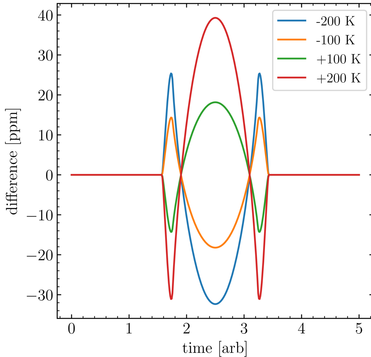
Figure 6. from Ben Cassese et al 2026 Astron. J. 171 doi:10.3847/1538-3881/ae3a81 https://dx.doi.org/10.3847/1538-3881/ae3a81 © 2026. The Author(s). Published by the American Astronomical Society.
