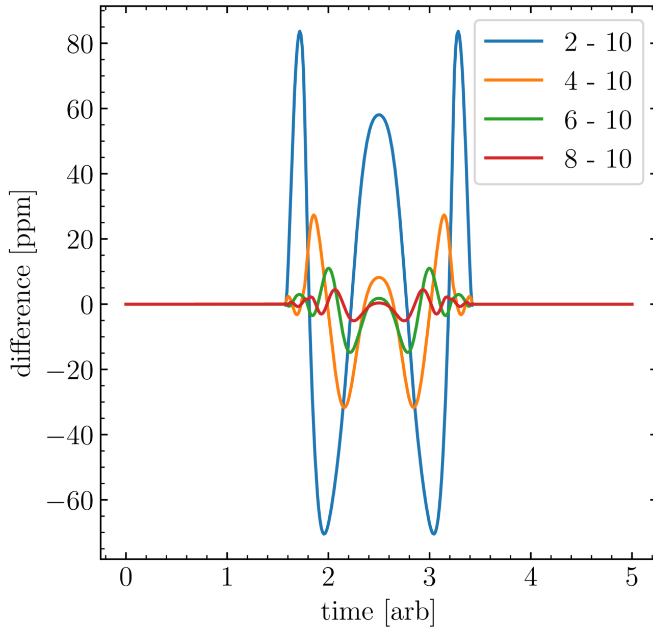
Figure 5. from Ben Cassese et al 2026 Astron. J. 171 doi:10.3847/1538-3881/ae3a81 https://dx.doi.org/10.3847/1538-3881/ae3a81 © 2026. The Author(s). Published by the American Astronomical Society.
