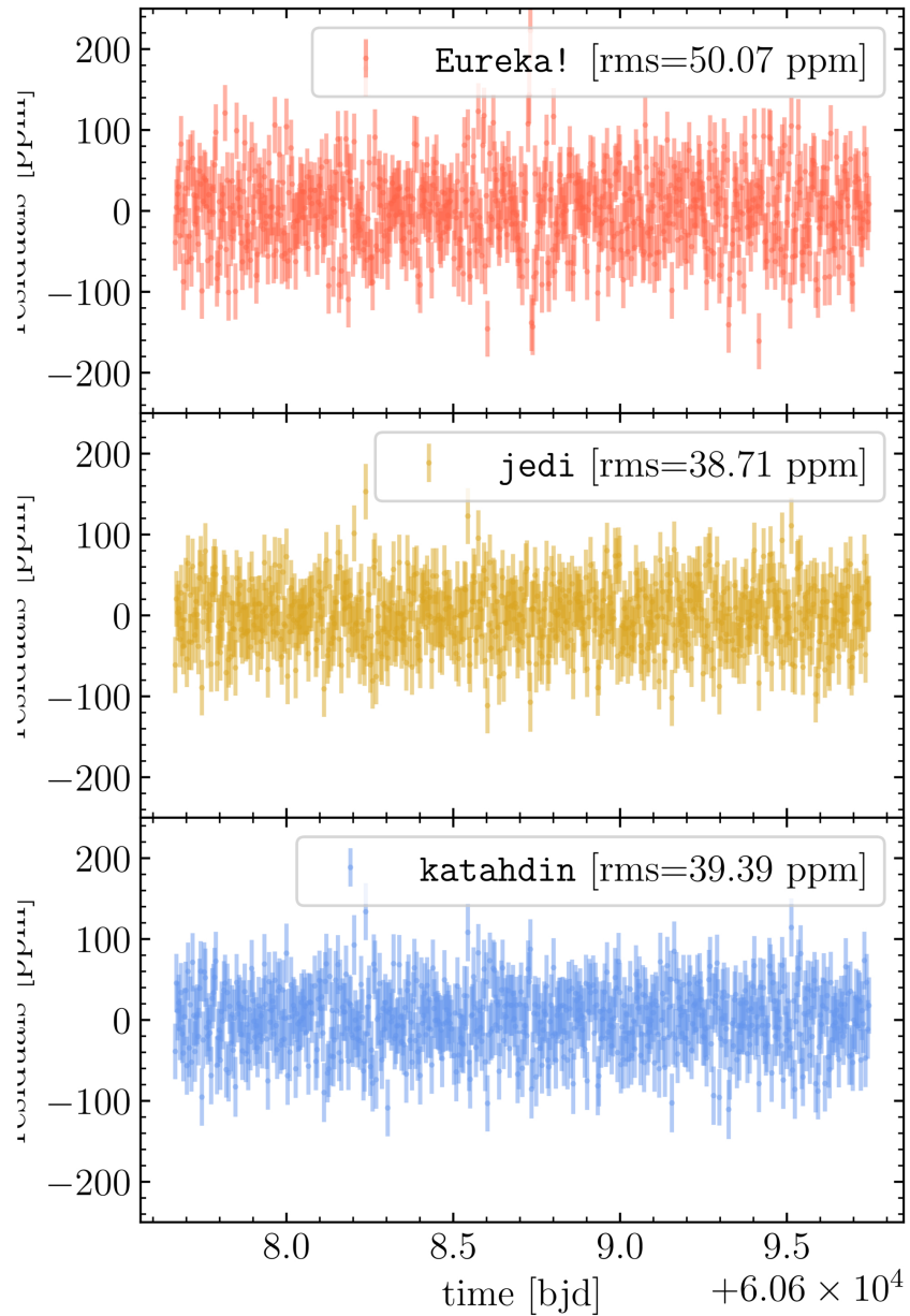
Figure 10. from Ben Cassese et al 2026 Astron. J. 171 doi:10.3847/1538-3881/ae3a81 https://dx.doi.org/10.3847/1538-3881/ae3a81 © 2026. The Author(s). Published by the American Astronomical Society.
