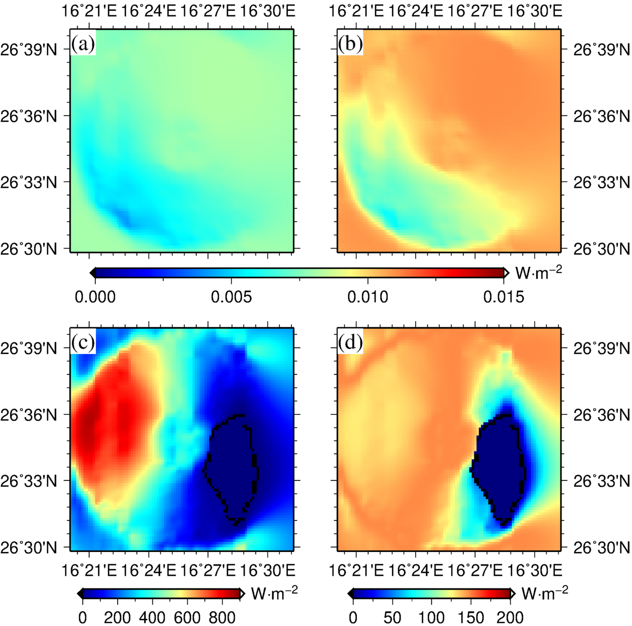
Figure 9. from Zhen Yang et al 2026 Astron. J. 171 doi:10.3847/1538-3881/ae38d6 https://dx.doi.org/10.3847/1538-3881/ae38d6 © 2026. The Author(s). Published by the American Astronomical Society.
