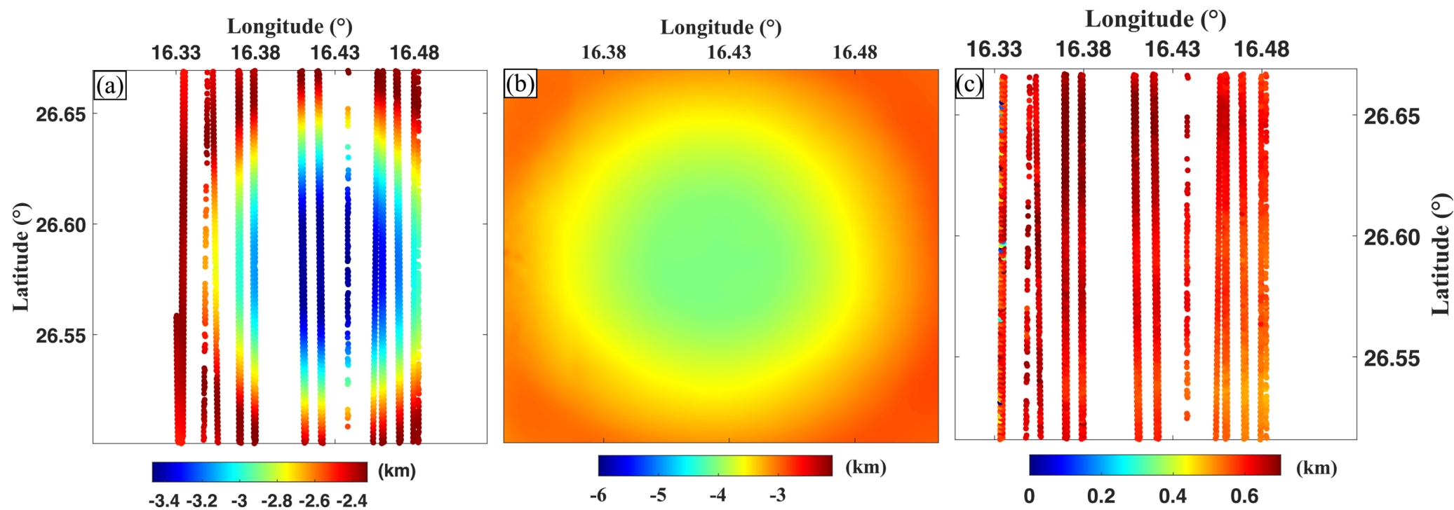
Figure 4. from Zhen Yang et al 2026 Astron. J. 171 doi:10.3847/1538-3881/ae38d6 https://dx.doi.org/10.3847/1538-3881/ae38d6 © 2026. The Author(s). Published by the American Astronomical Society.
