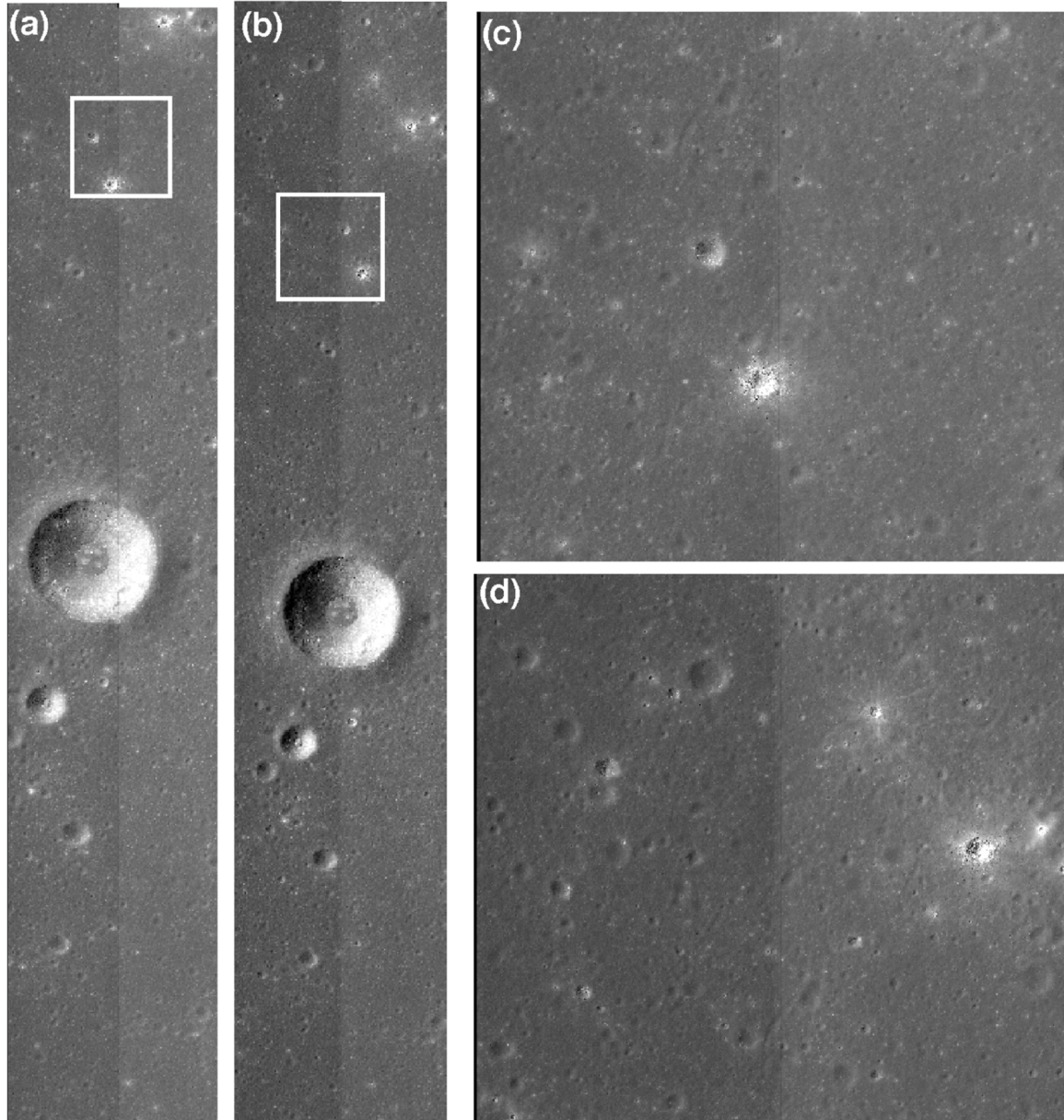
Figure 3. from Zhen Yang et al 2026 Astron. J. 171 doi:10.3847/1538-3881/ae38d6 https://dx.doi.org/10.3847/1538-3881/ae38d6 © 2026. The Author(s). Published by the American Astronomical Society.
