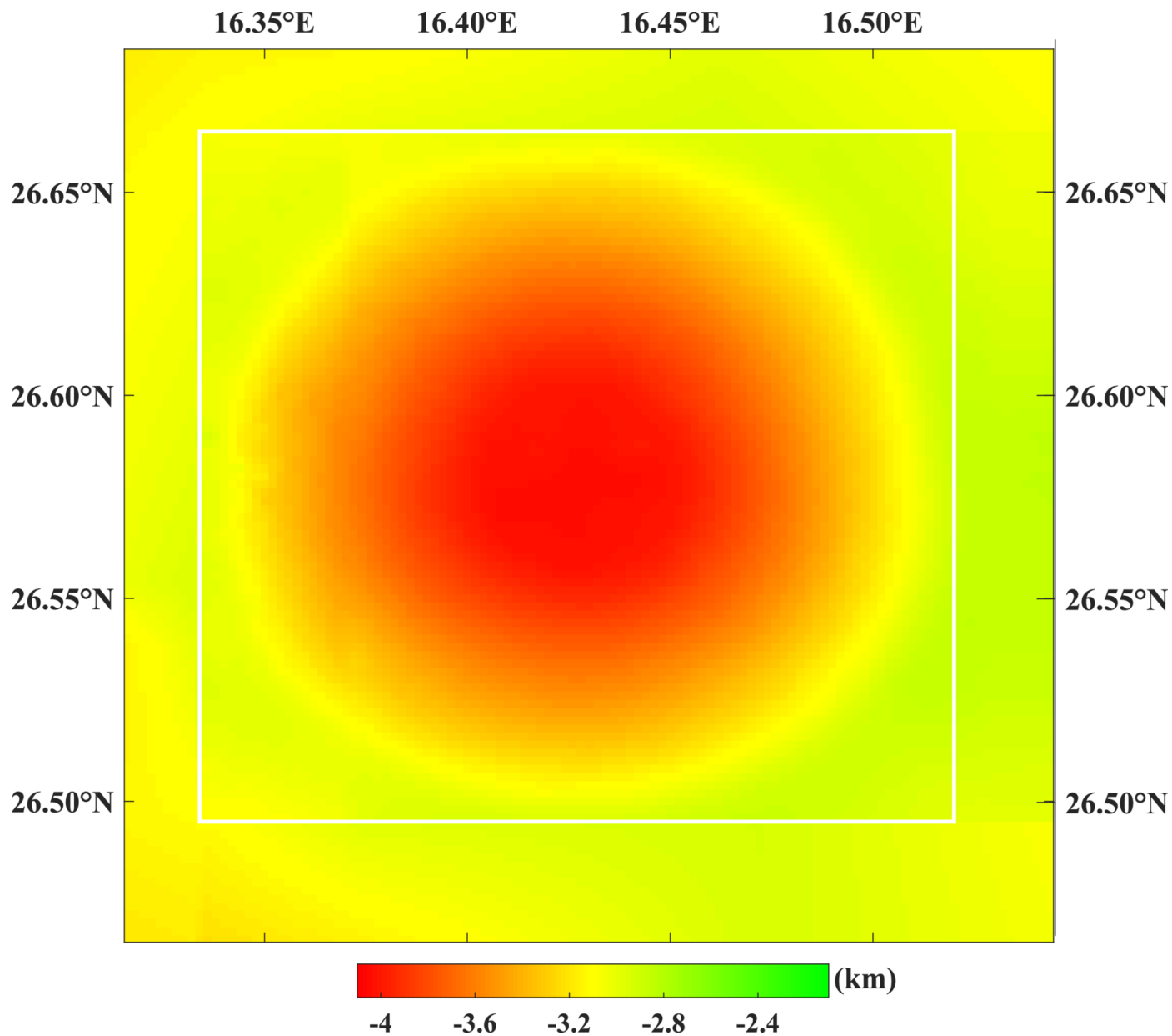
Figure 1. from Zhen Yang et al 2026 Astron. J. 171 doi:10.3847/1538-3881/ae38d6 https://dx.doi.org/10.3847/1538-3881/ae38d6 © 2026. The Author(s). Published by the American Astronomical Society.
