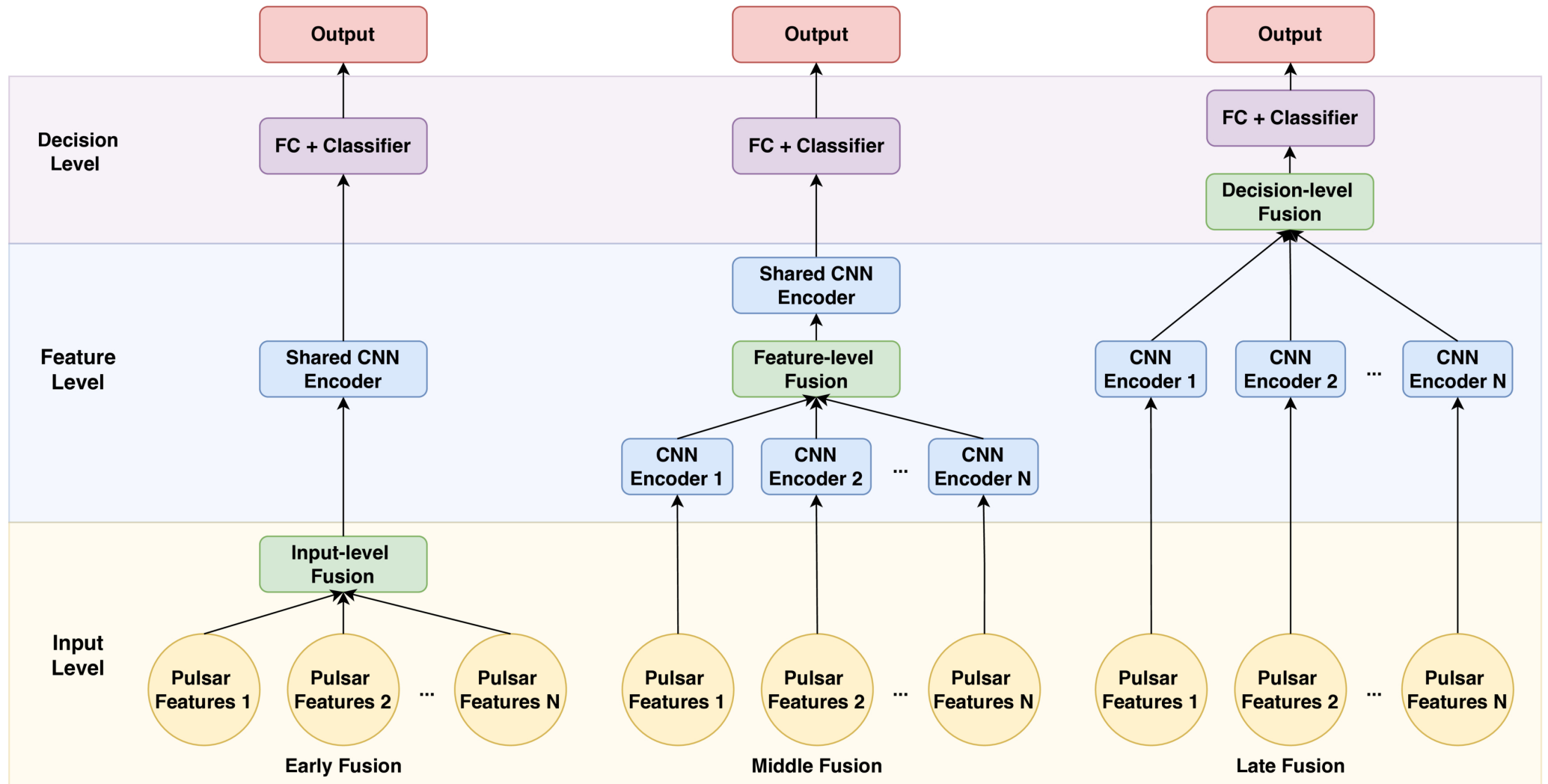
Figure 9. from Yining Song et al 2026 Astron. J. 171 doi:10.3847/1538-3881/ae38b2 https://dx.doi.org/10.3847/1538-3881/ae38b2 © 2026. The Author(s). Published by the American Astronomical Society.
