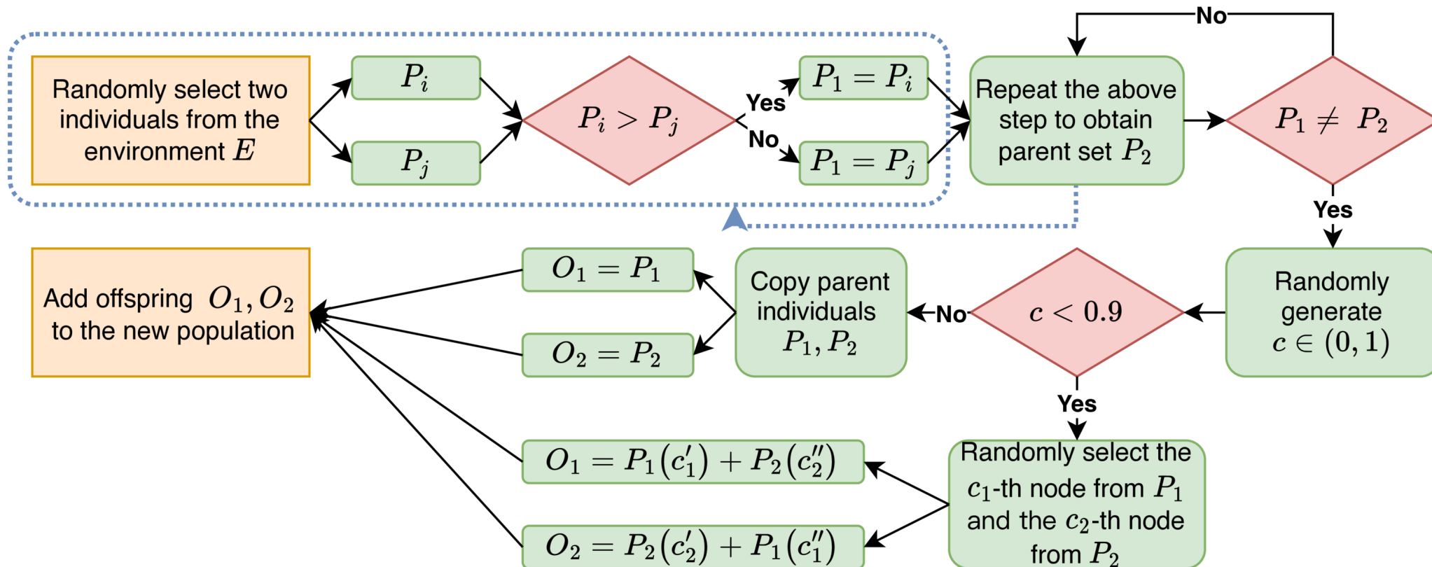
Figure 6. from Yining Song et al 2026 Astron. J. 171 doi:10.3847/1538-3881/ae38b2 https://dx.doi.org/10.3847/1538-3881/ae38b2 © 2026. The Author(s). Published by the American Astronomical Society.
