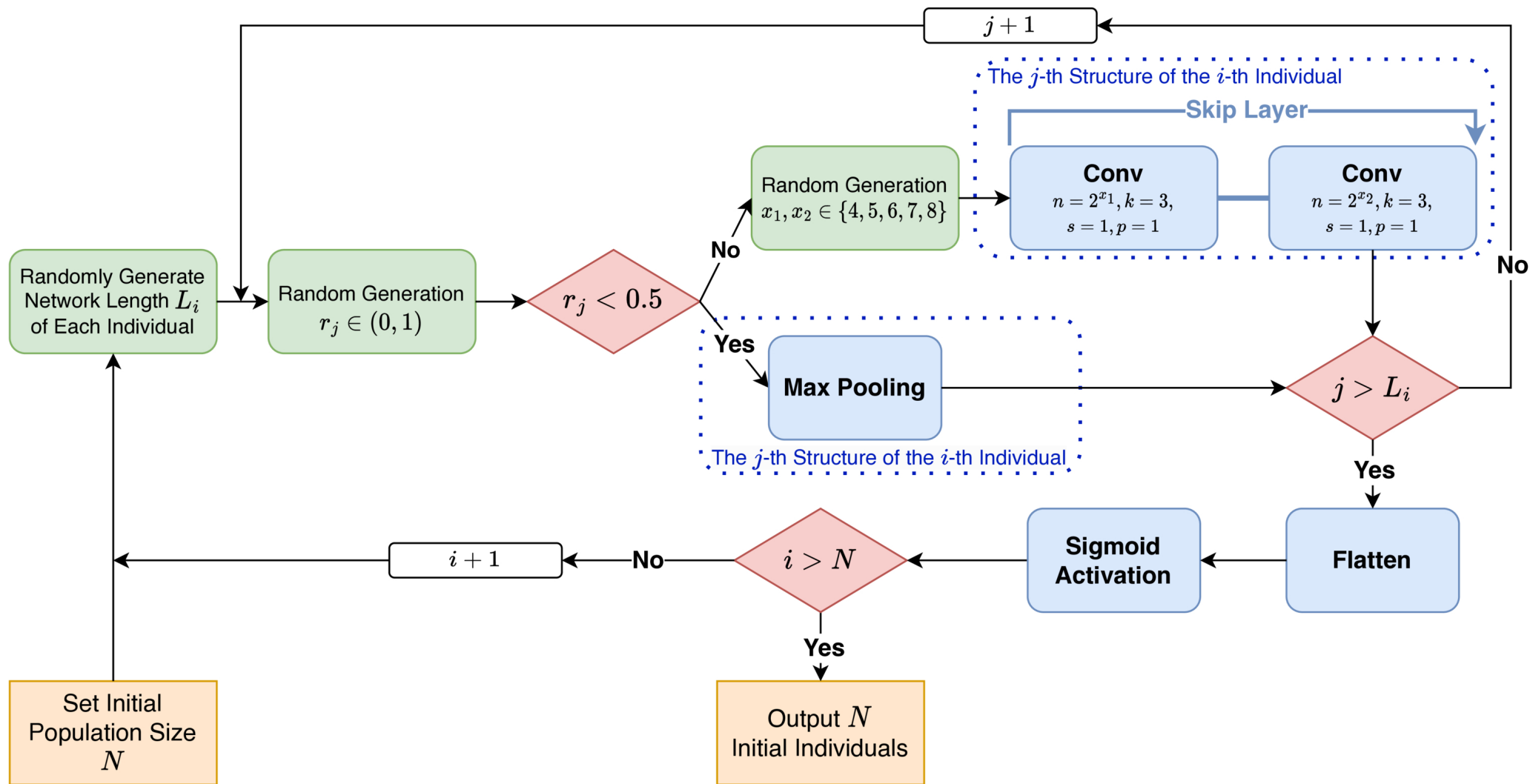
Figure 3. from Yining Song et al 2026 Astron. J. 171 doi:10.3847/1538-3881/ae38b2 https://dx.doi.org/10.3847/1538-3881/ae38b2 © 2026. The Author(s). Published by the American Astronomical Society.
