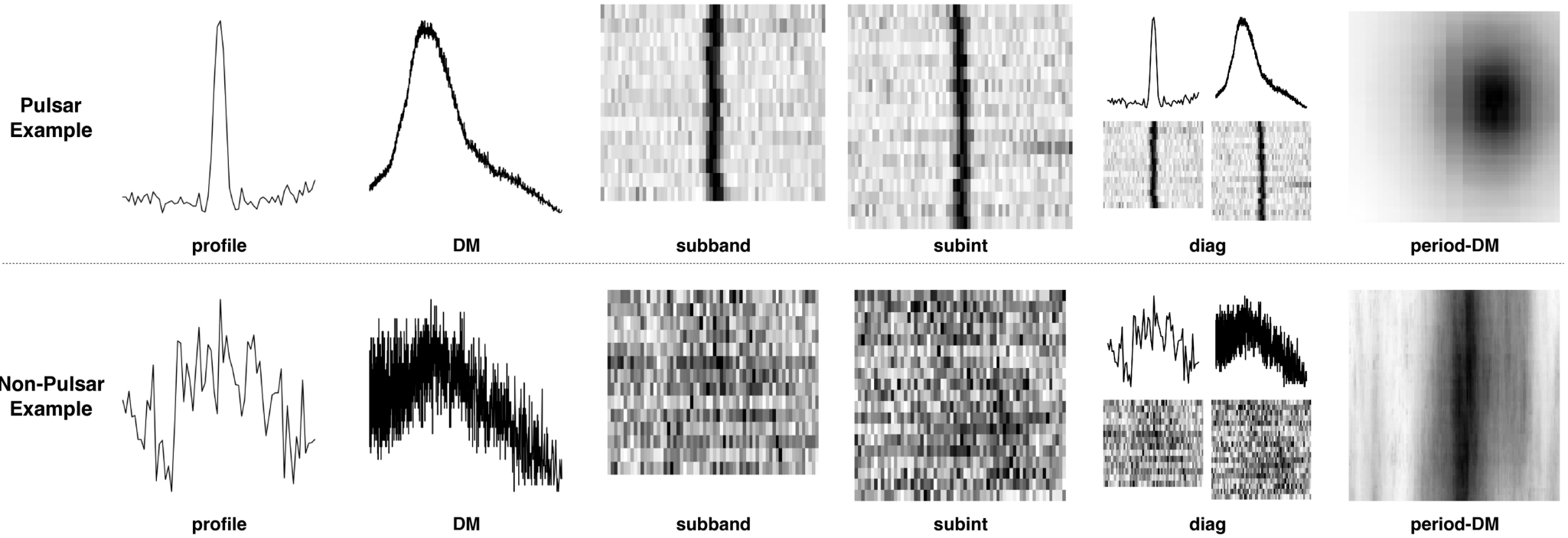
Figure 11. from Yining Song et al 2026 Astron. J. 171 doi:10.3847/1538-3881/ae38b2 https://dx.doi.org/10.3847/1538-3881/ae38b2 © 2026. The Author(s). Published by the American Astronomical Society.
