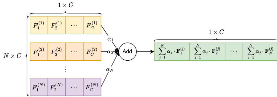
(1) Addition Fusion
