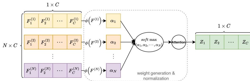
(3) Attention Fusion
