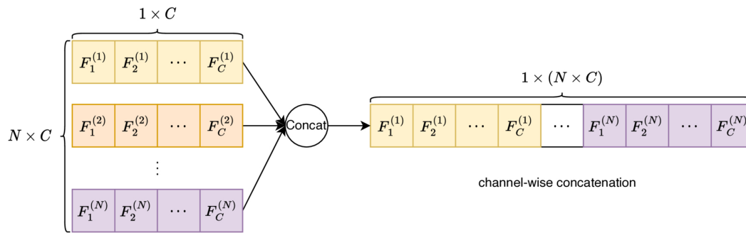
(2) Concatenation Fusion
