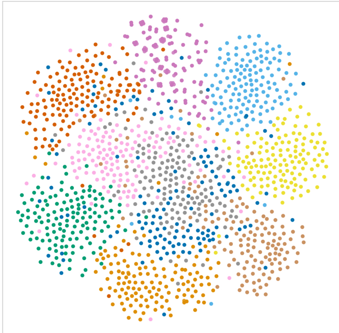
Figure 5. from Handa Cai and Weibin Chen 2026 Astron. J. 171 doi:10.3847/1538-3881/ae37eb https://dx.doi.org/10.3847/1538-3881/ae37eb © 2026. The Author(s). Published by the American Astronomical Society.
