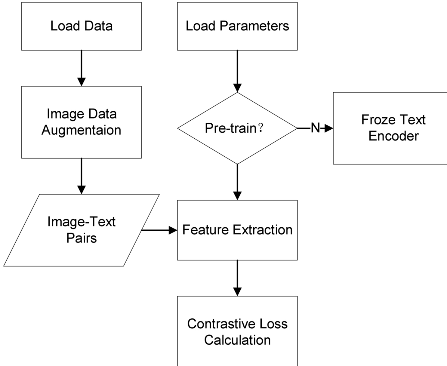
Figure 2. from Handa Cai and Weibin Chen 2026 Astron. J. 171 doi:10.3847/1538-3881/ae37eb https://dx.doi.org/10.3847/1538-3881/ae37eb © 2026. The Author(s). Published by the American Astronomical Society.
