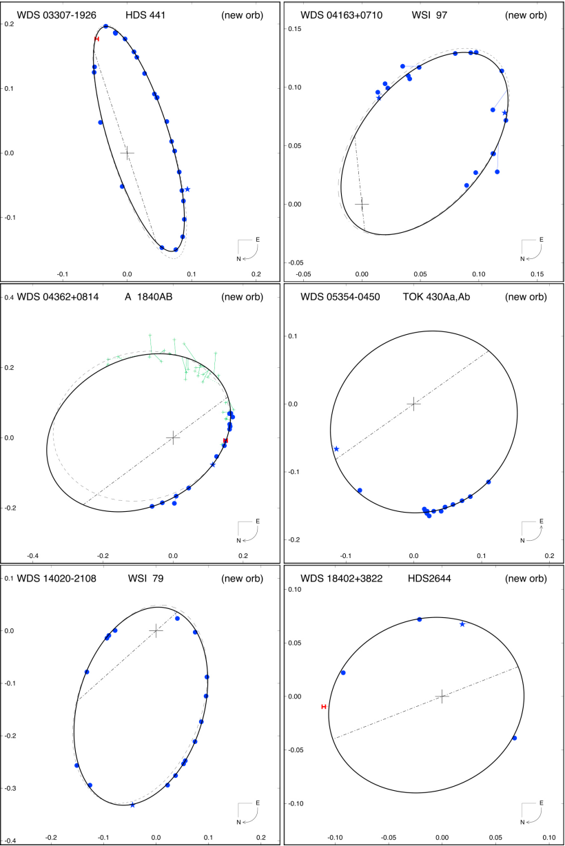
Figure 1. from Brian D. Mason and William I. Hartkopf 2026 Astron. J. 171 doi:10.3847/1538-3881/ae3748 https://dx.doi.org/10.3847/1538-3881/ae3748 © 2026. The Author(s). Published by the American Astronomical Society.
