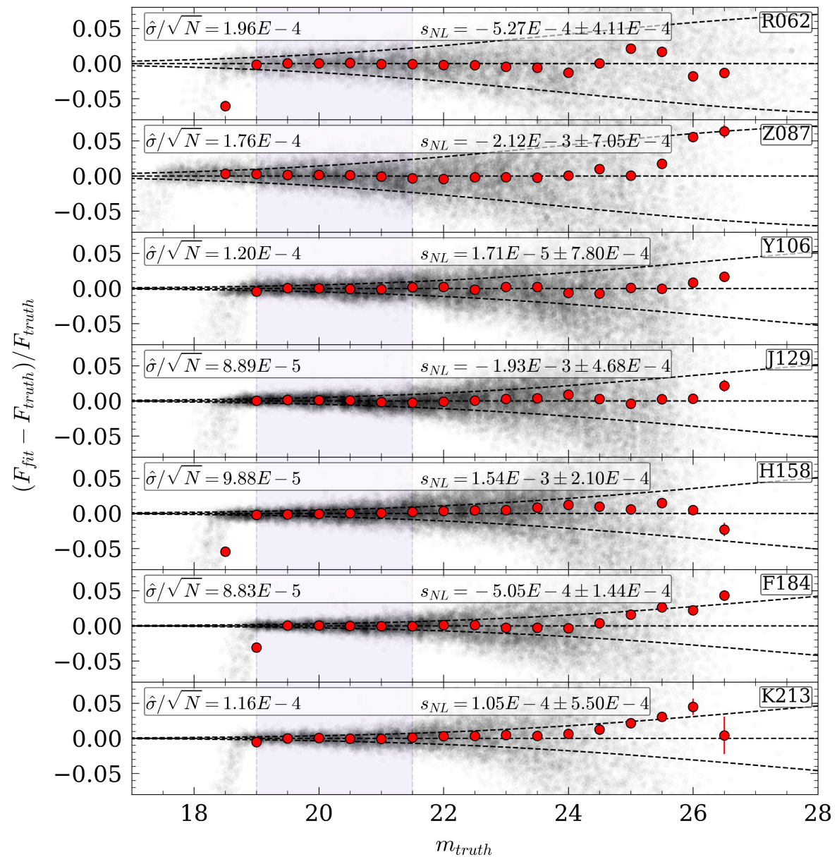
Figure 2. from L. Aldoroty et al 2026 Astron. J. 171 doi:10.3847/1538-3881/ae3714 https://dx.doi.org/10.3847/1538-3881/ae3714 © 2026. The Author(s). Published by the American Astronomical Society.
