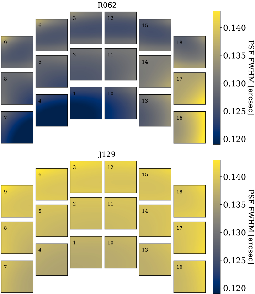
Figure 1. from L. Aldoroty et al 2026 Astron. J. 171 doi:10.3847/1538-3881/ae3714 https://dx.doi.org/10.3847/1538-3881/ae3714 © 2026. The Author(s). Published by the American Astronomical Society.
