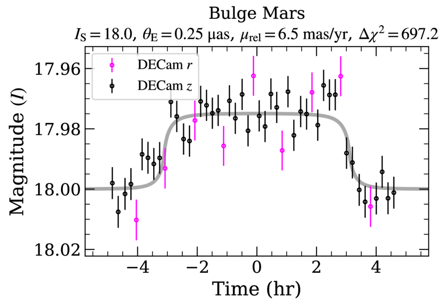
Figure 7. from Hongjing Yang et al 2026 Astron. J. 171 doi:10.3847/1538-3881/ae36ac https://dx.doi.org/10.3847/1538-3881/ae36ac © 2026. The Author(s). Published by the American Astronomical Society.
