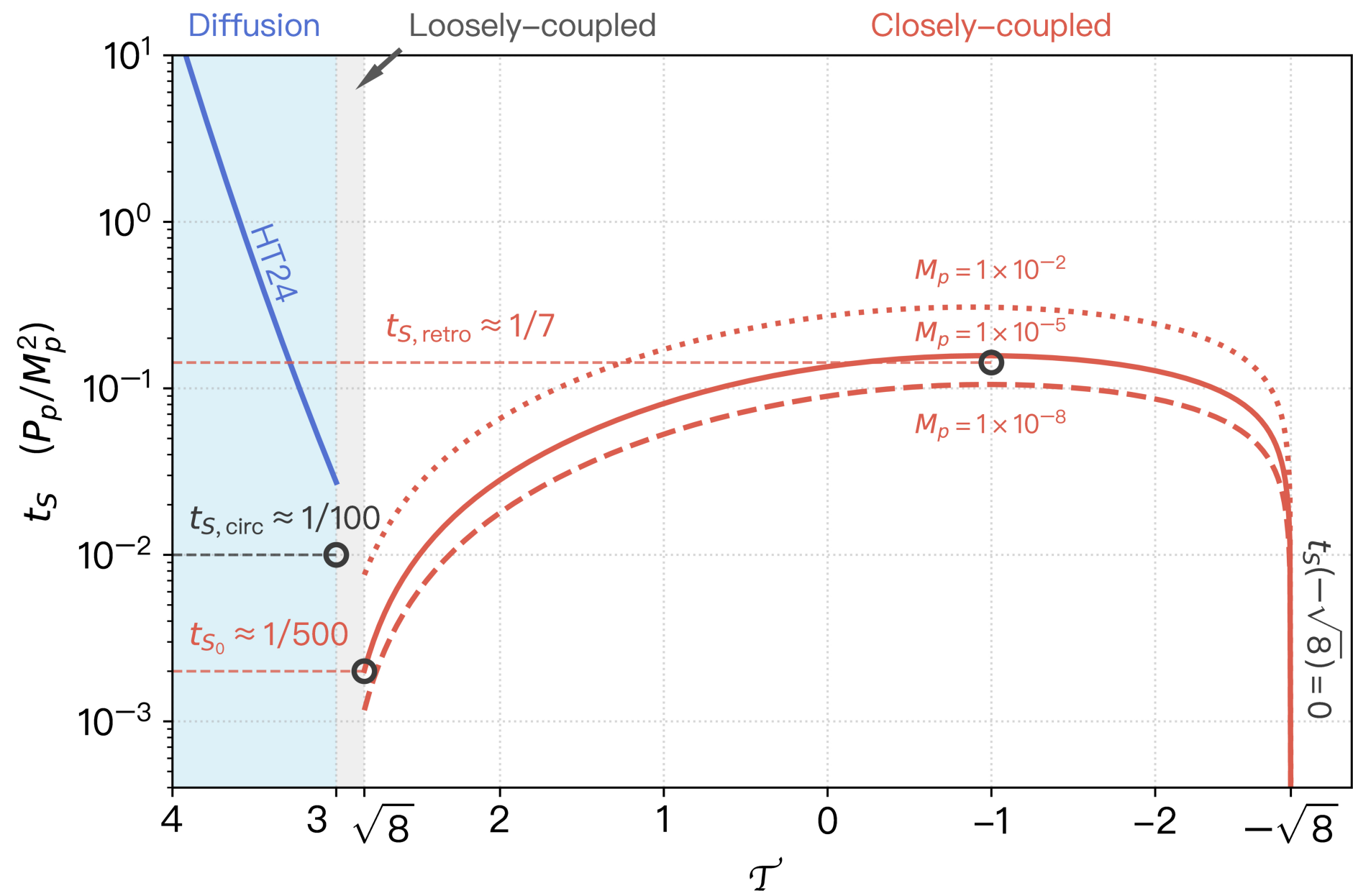
Figure 7. from Yukun Huang et al 2026 Astron. J. 171 doi:10.3847/1538-3881/ae3566 https://dx.doi.org/10.3847/1538-3881/ae3566 © 2026. The Author(s). Published by the American Astronomical Society.
