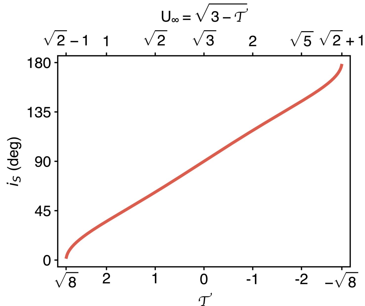
Figure 6. from Yukun Huang et al 2026 Astron. J. 171 doi:10.3847/1538-3881/ae3566 https://dx.doi.org/10.3847/1538-3881/ae3566 © 2026. The Author(s). Published by the American Astronomical Society.
