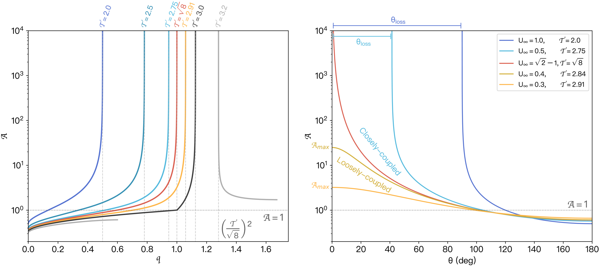
Figure 2. from Yukun Huang et al 2026 Astron. J. 171 doi:10.3847/1538-3881/ae3566 https://dx.doi.org/10.3847/1538-3881/ae3566 © 2026. The Author(s). Published by the American Astronomical Society.
