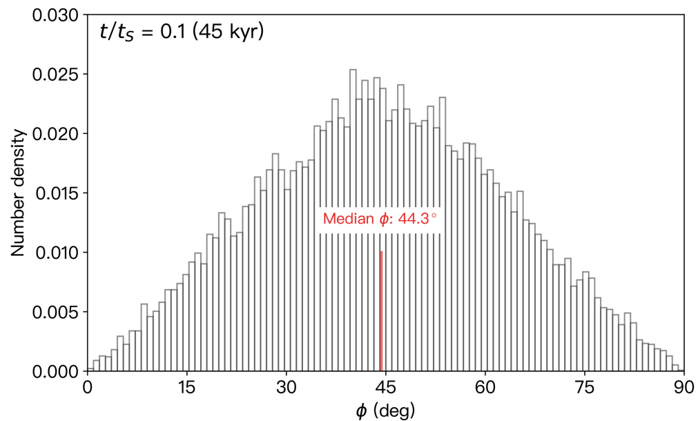
Figure 14. from Yukun Huang et al 2026 Astron. J. 171 doi:10.3847/1538-3881/ae3566 https://dx.doi.org/10.3847/1538-3881/ae3566 © 2026. The Author(s). Published by the American Astronomical Society.
