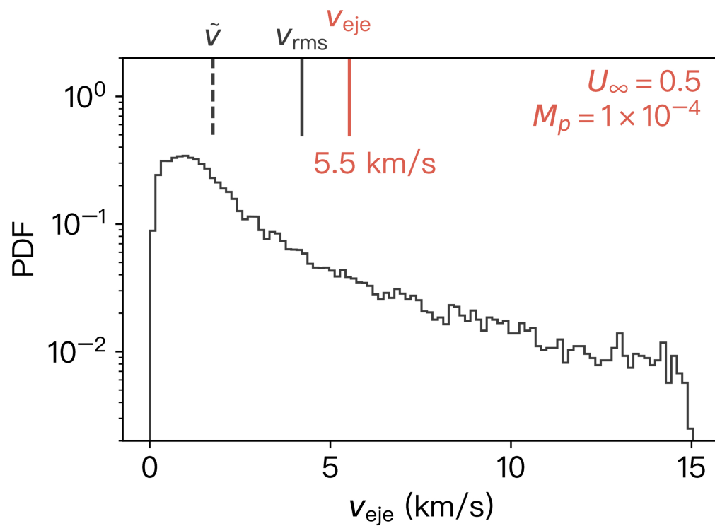
Figure 12. from Yukun Huang et al 2026 Astron. J. 171 doi:10.3847/1538-3881/ae3566 https://dx.doi.org/10.3847/1538-3881/ae3566 © 2026. The Author(s). Published by the American Astronomical Society.
