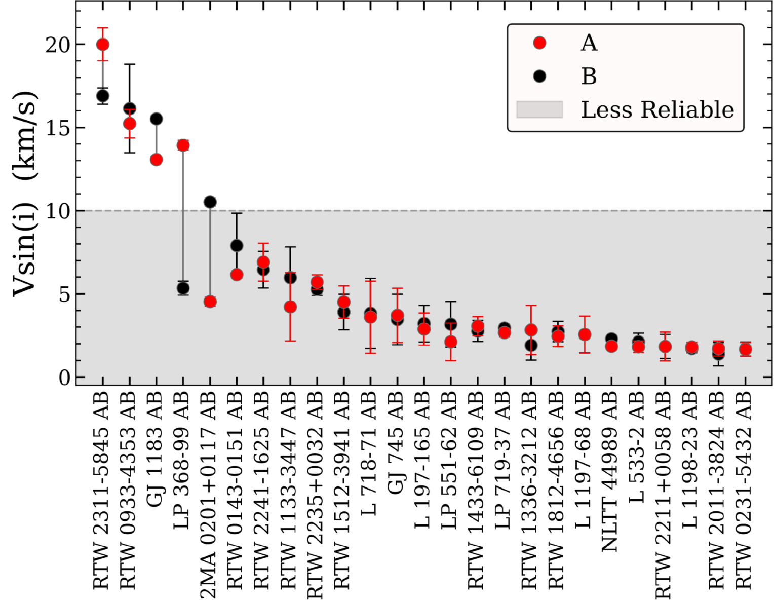
Figure 4. from Andrew A. Couperus et al 2026 Astron. J. 171 doi:10.3847/1538-3881/ae34ad https://dx.doi.org/10.3847/1538-3881/ae34ad © 2026. The Author(s). Published by the American Astronomical Society.
