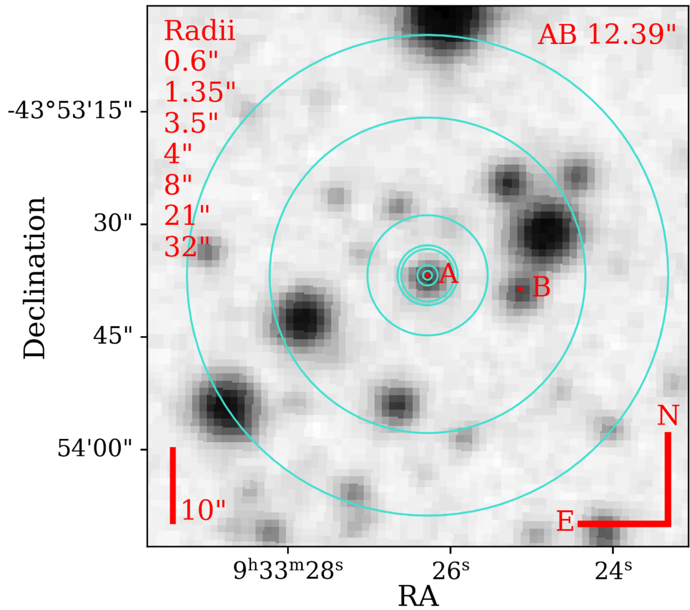
Figure 2. from Andrew A. Couperus et al 2026 Astron. J. 171 doi:10.3847/1538-3881/ae34ad https://dx.doi.org/10.3847/1538-3881/ae34ad © 2026. The Author(s). Published by the American Astronomical Society.
