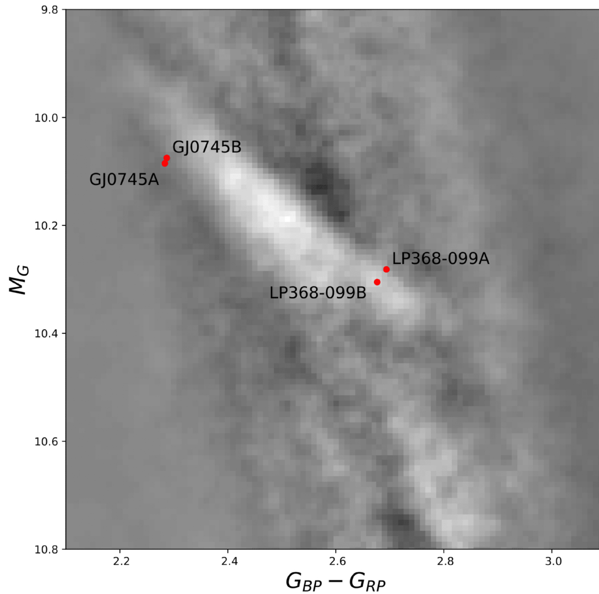
Figure 18. from Andrew A. Couperus et al 2026 Astron. J. 171 doi:10.3847/1538-3881/ae34ad https://dx.doi.org/10.3847/1538-3881/ae34ad © 2026. The Author(s). Published by the American Astronomical Society.
