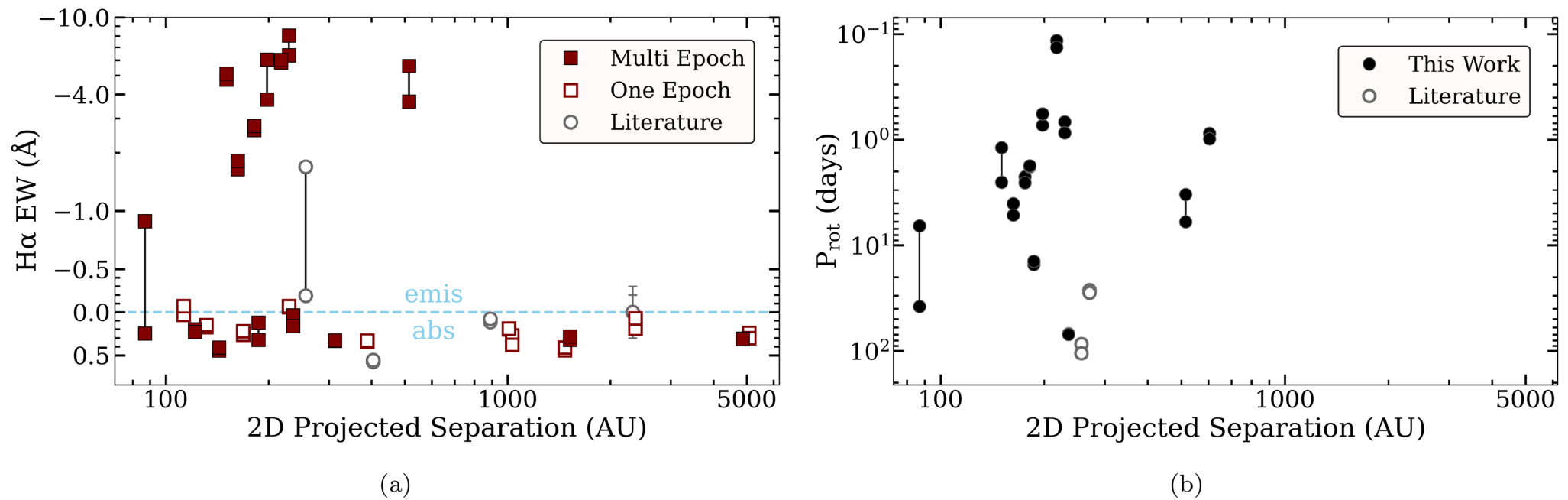
Figure 16. from Andrew A. Couperus et al 2026 Astron. J. 171 doi:10.3847/1538-3881/ae34ad https://dx.doi.org/10.3847/1538-3881/ae34ad © 2026. The Author(s). Published by the American Astronomical Society.
