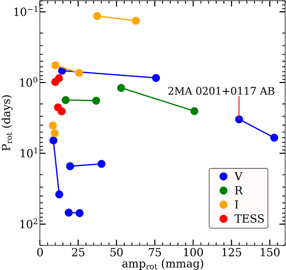
Figure 15. from Andrew A. Couperus et al 2026 Astron. J. 171 doi:10.3847/1538-3881/ae34ad https://dx.doi.org/10.3847/1538-3881/ae34ad © 2026. The Author(s). Published by the American Astronomical Society.
