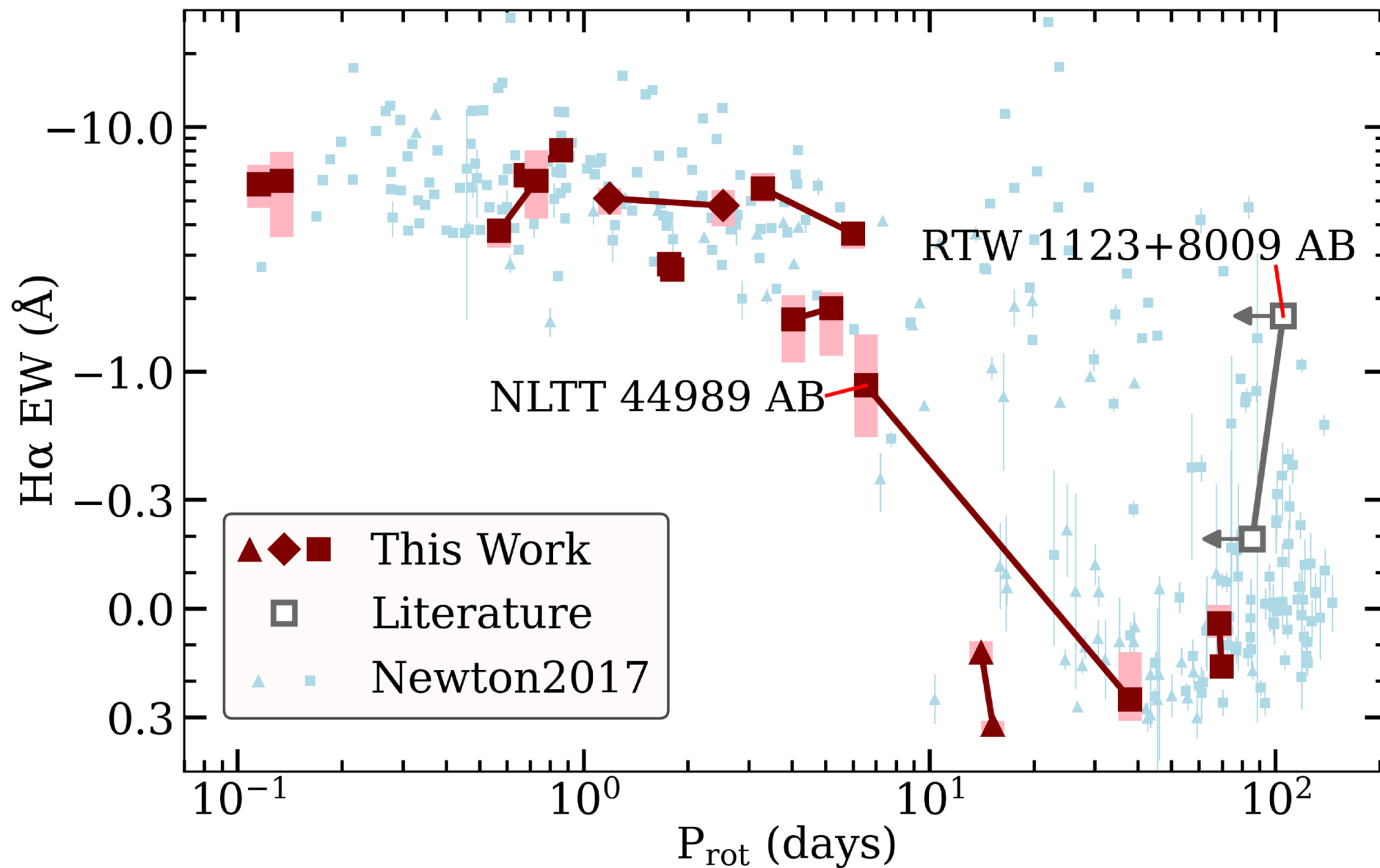
Figure 14. from Andrew A. Couperus et al 2026 Astron. J. 171 doi:10.3847/1538-3881/ae34ad https://dx.doi.org/10.3847/1538-3881/ae34ad © 2026. The Author(s). Published by the American Astronomical Society.
