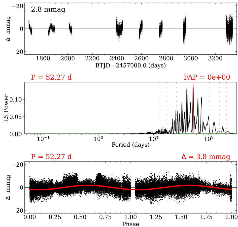
Figure 12. from Andrew A. Couperus et al 2026 Astron. J. 171 doi:10.3847/1538-3881/ae34ad https://dx.doi.org/10.3847/1538-3881/ae34ad © 2026. The Author(s). Published by the American Astronomical Society.
