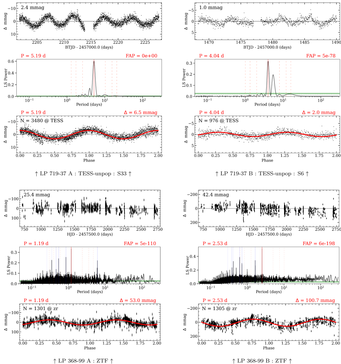
Figure 11. from Andrew A. Couperus et al 2026 Astron. J. 171 doi:10.3847/1538-3881/ae34ad https://dx.doi.org/10.3847/1538-3881/ae34ad © 2026. The Author(s). Published by the American Astronomical Society.
