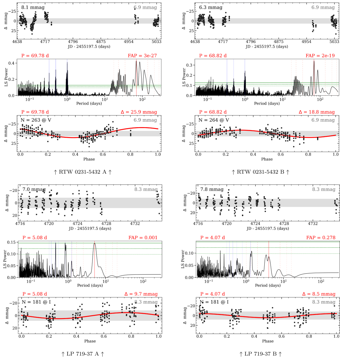
Figure 10. from Andrew A. Couperus et al 2026 Astron. J. 171 doi:10.3847/1538-3881/ae34ad https://dx.doi.org/10.3847/1538-3881/ae34ad © 2026. The Author(s). Published by the American Astronomical Society.
