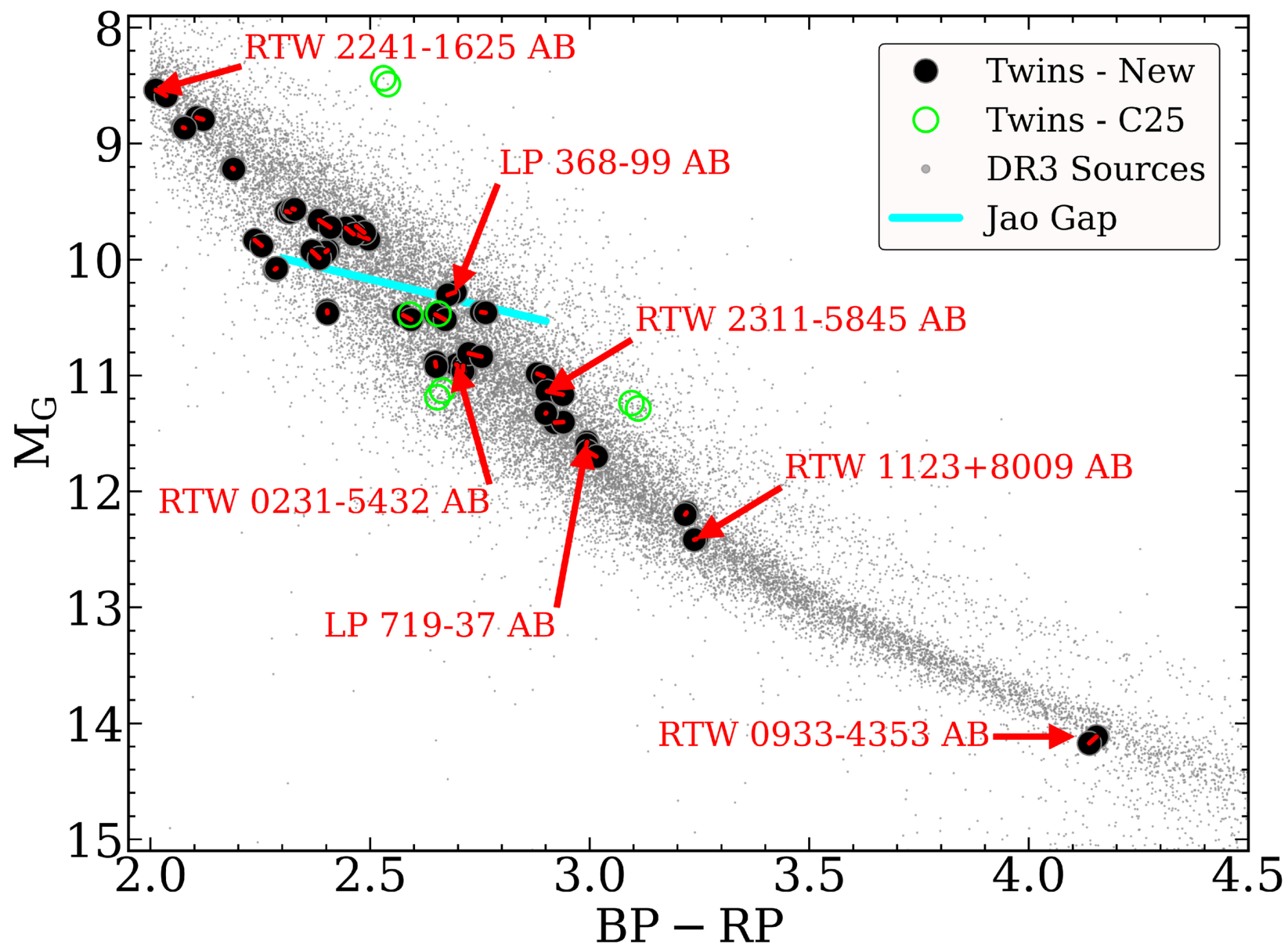
Figure 1. from Andrew A. Couperus et al 2026 Astron. J. 171 doi:10.3847/1538-3881/ae34ad https://dx.doi.org/10.3847/1538-3881/ae34ad © 2026. The Author(s). Published by the American Astronomical Society.
