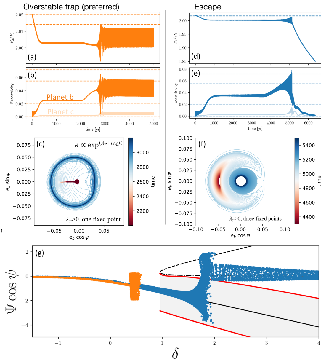
Figure 9. from Mu-Tian Wang et al 2026 Astron. J. 171 doi:10.3847/1538-3881/ae346d https://dx.doi.org/10.3847/1538-3881/ae346d © 2026. The Author(s). Published by the American Astronomical Society.
