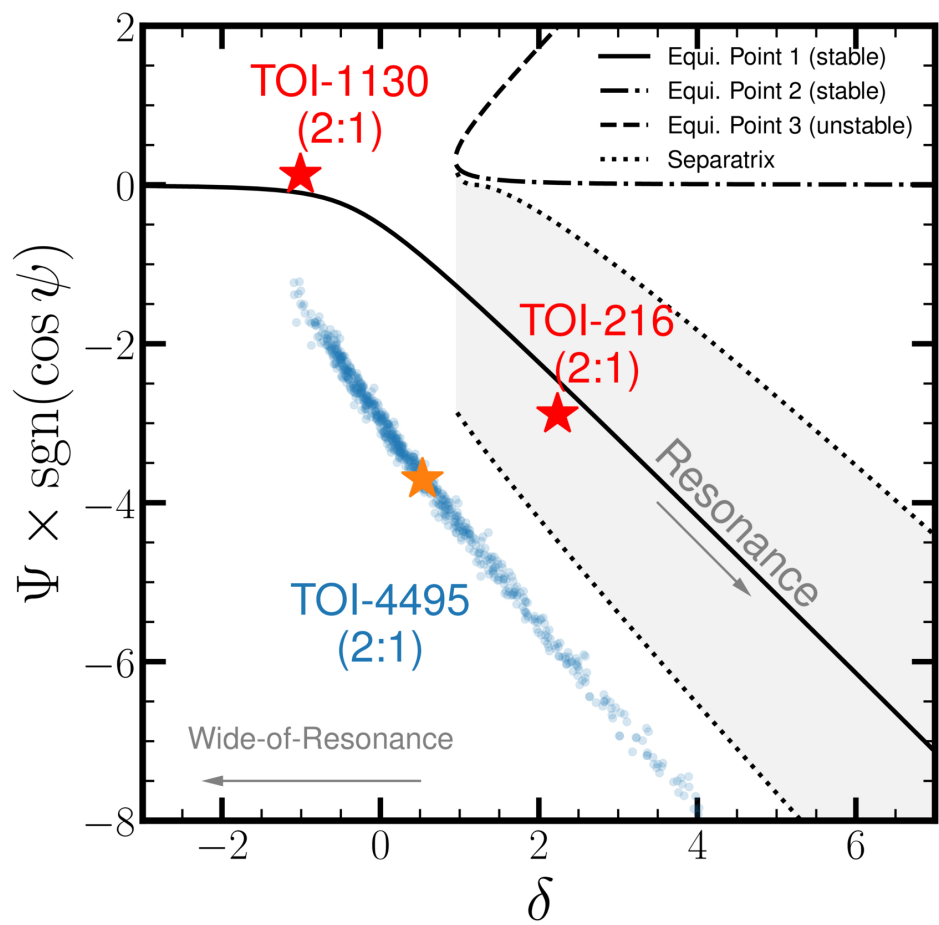
Figure 7. from Mu-Tian Wang et al 2026 Astron. J. 171 doi:10.3847/1538-3881/ae346d https://dx.doi.org/10.3847/1538-3881/ae346d © 2026. The Author(s). Published by the American Astronomical Society.
