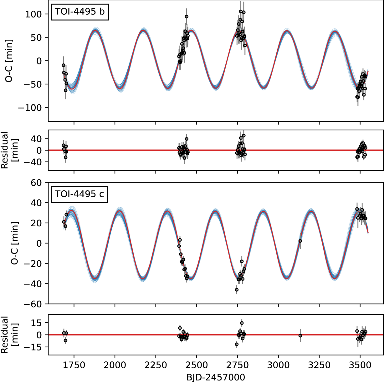
Figure 5. from Mu-Tian Wang et al 2026 Astron. J. 171 doi:10.3847/1538-3881/ae346d https://dx.doi.org/10.3847/1538-3881/ae346d © 2026. The Author(s). Published by the American Astronomical Society.
