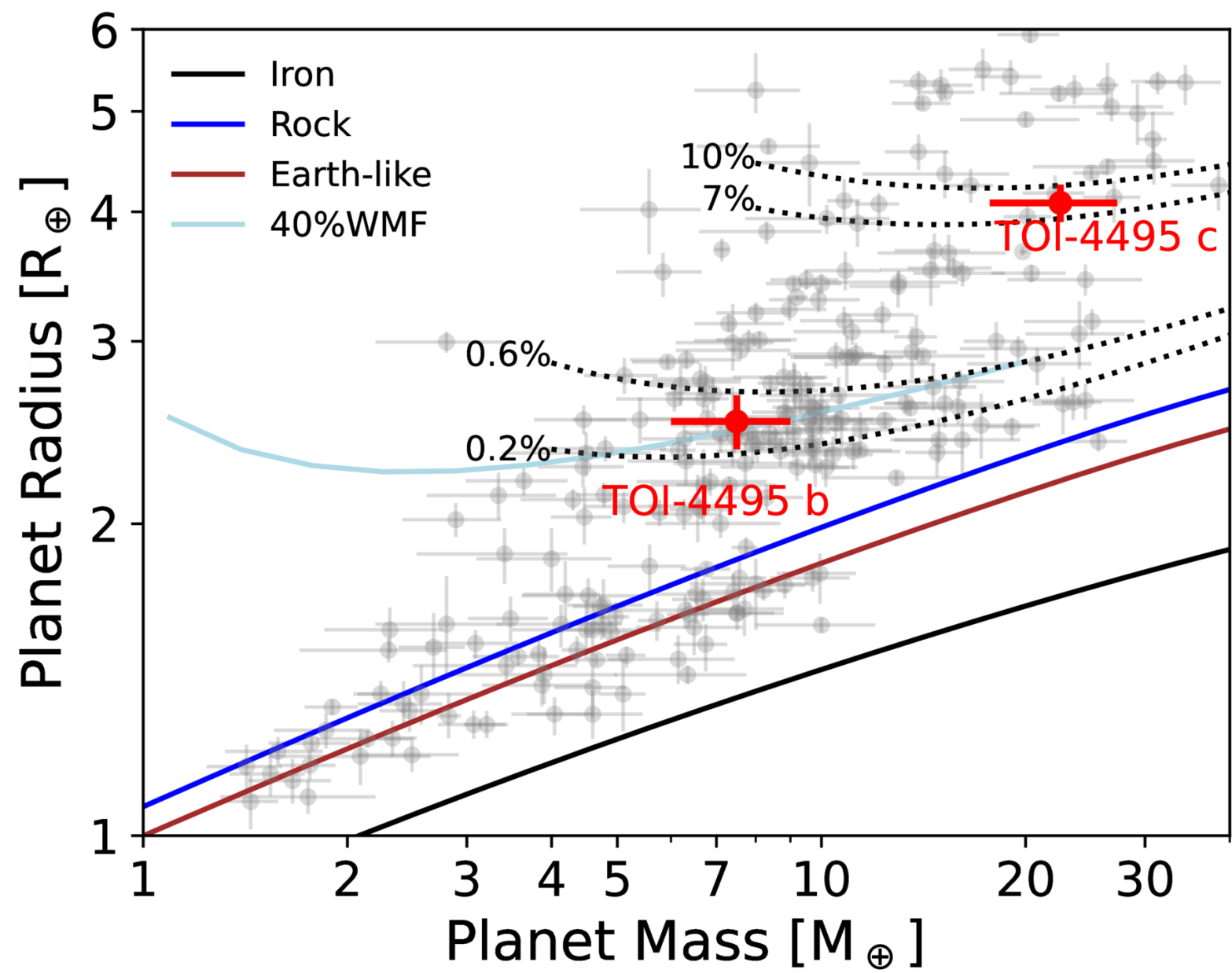
Figure 4. from Mu-Tian Wang et al 2026 Astron. J. 171 doi:10.3847/1538-3881/ae346d https://dx.doi.org/10.3847/1538-3881/ae346d © 2026. The Author(s). Published by the American Astronomical Society.
