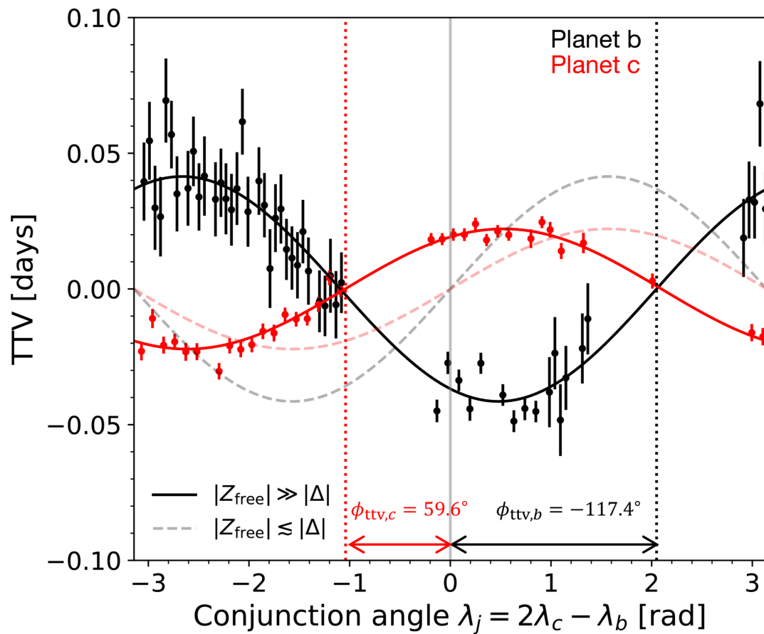
Figure 3. from Mu-Tian Wang et al 2026 Astron. J. 171 doi:10.3847/1538-3881/ae346d https://dx.doi.org/10.3847/1538-3881/ae346d © 2026. The Author(s). Published by the American Astronomical Society.
