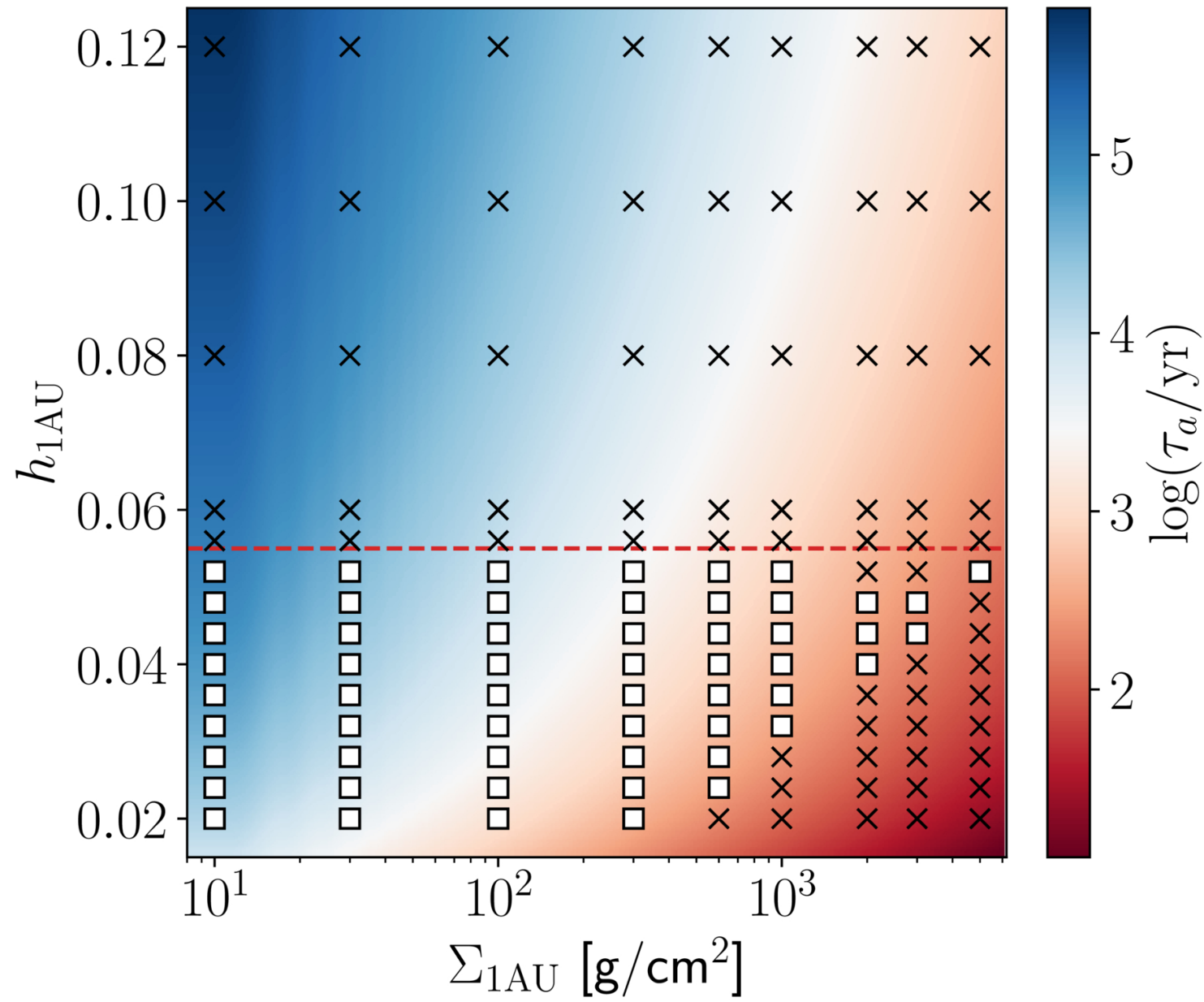
Figure 10. from Mu-Tian Wang et al 2026 Astron. J. 171 doi:10.3847/1538-3881/ae346d https://dx.doi.org/10.3847/1538-3881/ae346d © 2026. The Author(s). Published by the American Astronomical Society.
