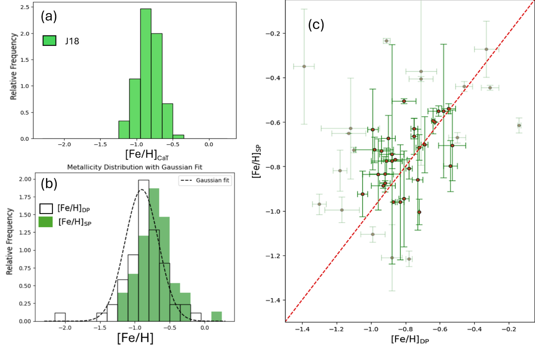
Figure 5. from Joanne Hughes et al 2026 Astron. J. 171 doi:10.3847/1538-3881/ae32f7 https://dx.doi.org/10.3847/1538-3881/ae32f7 © 2026. The Author(s). Published by the American Astronomical Society.
