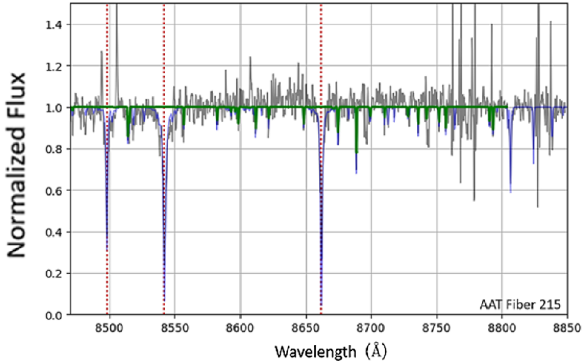
Figure 3. from Joanne Hughes et al 2026 Astron. J. 171 doi:10.3847/1538-3881/ae32f7 https://dx.doi.org/10.3847/1538-3881/ae32f7 © 2026. The Author(s). Published by the American Astronomical Society.
