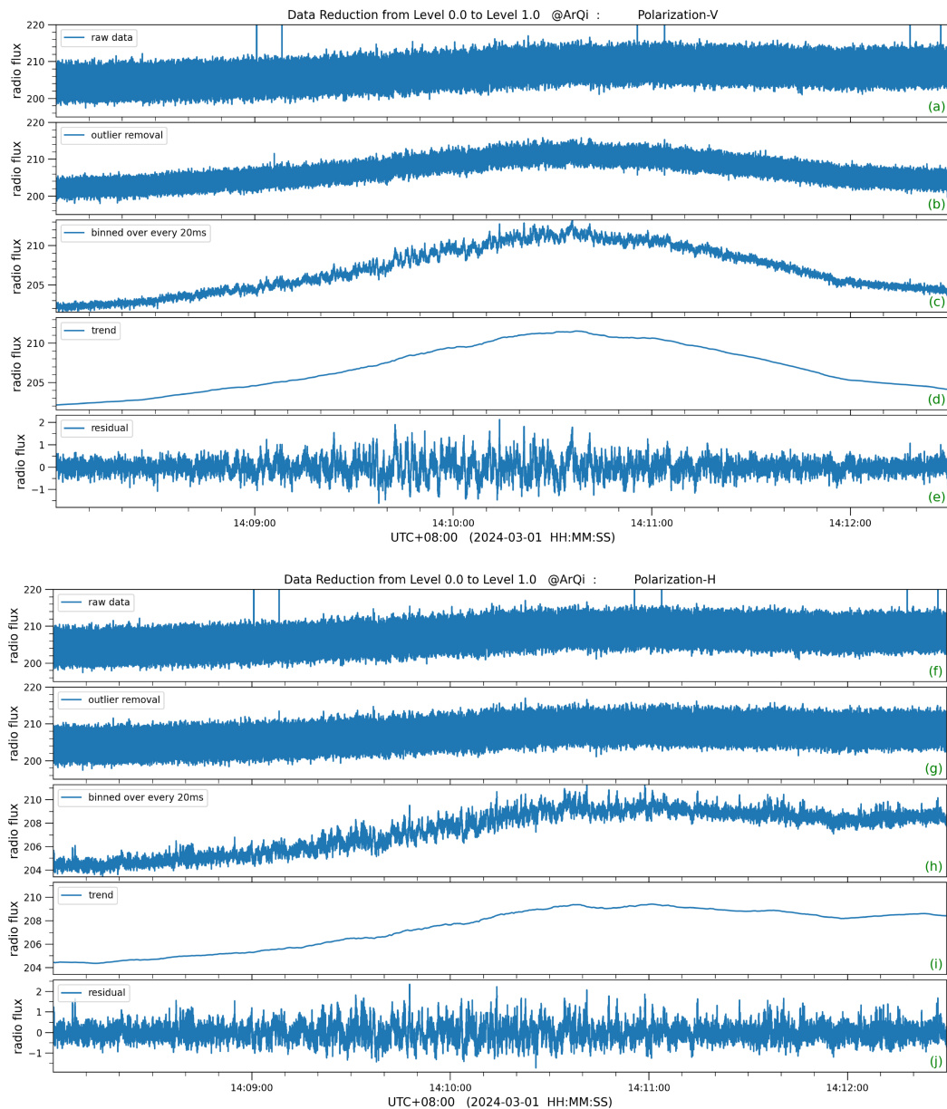
Figure 1. from Ming Xiong et al 2026 Astron. J. 171 doi:10.3847/1538-3881/ae328d https://dx.doi.org/10.3847/1538-3881/ae328d © 2026. The Author(s). Published by the American Astronomical Society.
