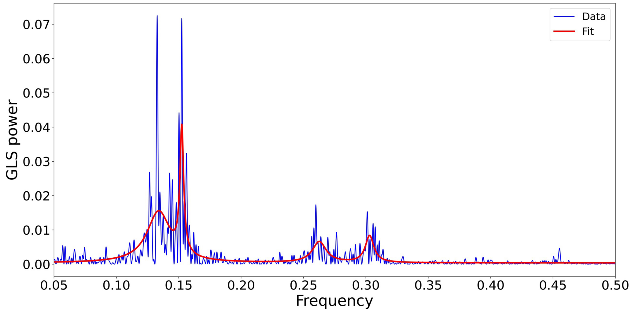
Figure 7. from Xiao-Hui Xu et al 2026 Astron. J. 171 doi:10.3847/1538-3881/ae3242 https://dx.doi.org/10.3847/1538-3881/ae3242 © 2026. The Author(s). Published by the American Astronomical Society.
