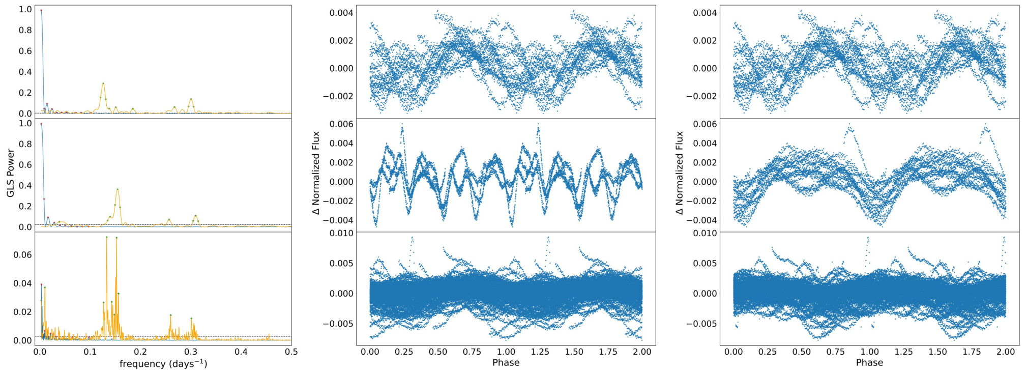
Figure 6. from Xiao-Hui Xu et al 2026 Astron. J. 171 doi:10.3847/1538-3881/ae3242 https://dx.doi.org/10.3847/1538-3881/ae3242 © 2026. The Author(s). Published by the American Astronomical Society.
