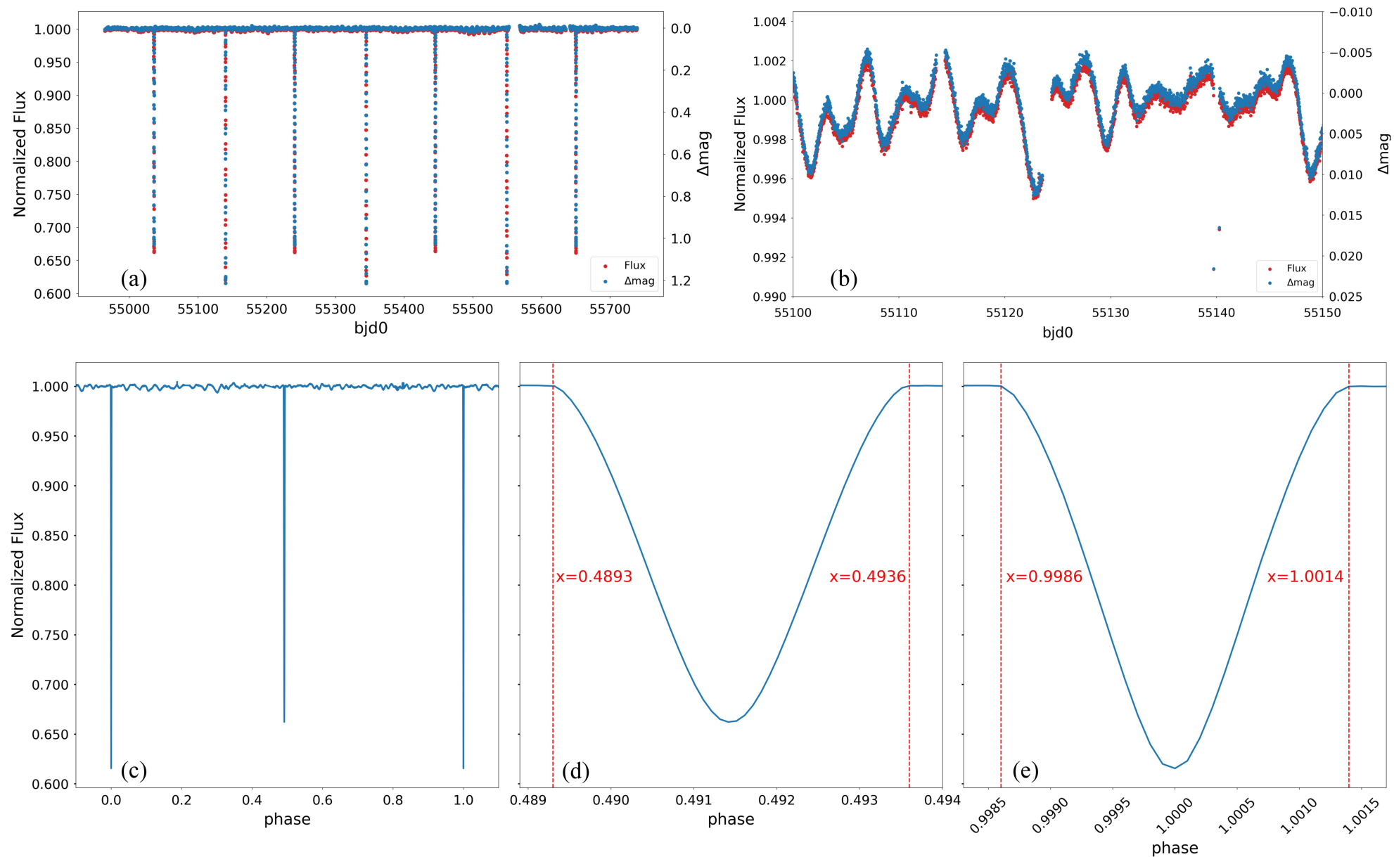
Figure 1. from Xiao-Hui Xu et al 2026 Astron. J. 171 doi:10.3847/1538-3881/ae3242 https://dx.doi.org/10.3847/1538-3881/ae3242 © 2026. The Author(s). Published by the American Astronomical Society.
