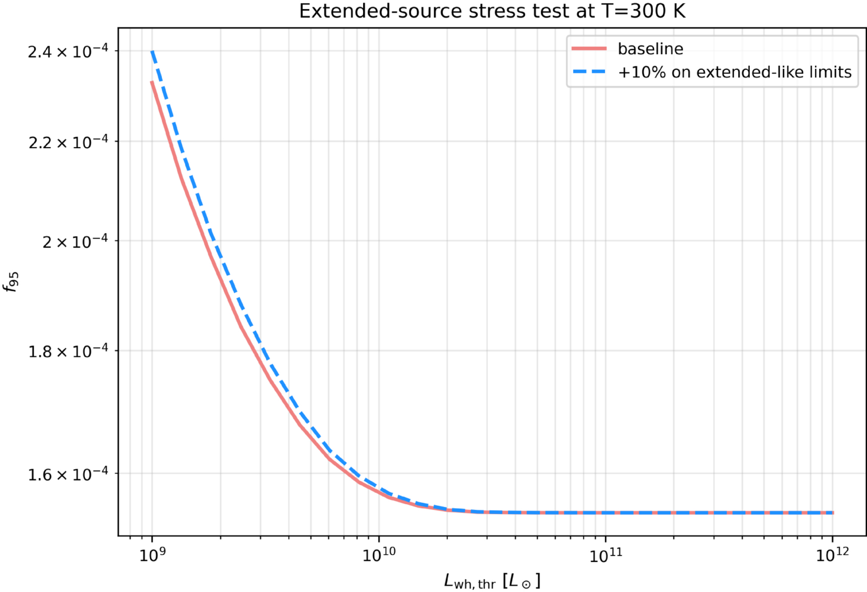
Figure 9. from Bo-Lun Huang et al 2026 Astron. J. 171 doi:10.3847/1538-3881/ae31e9 https://dx.doi.org/10.3847/1538-3881/ae31e9 © 2026. The Author(s). Published by the American Astronomical Society.
