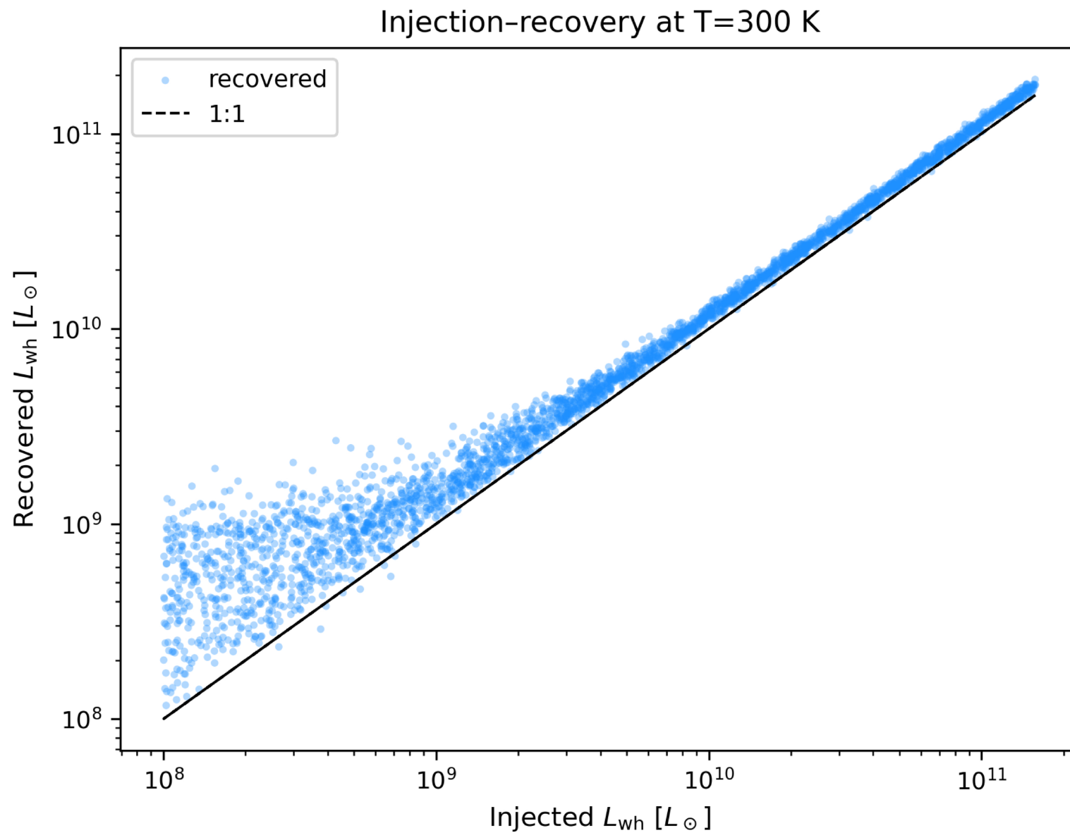
Figure 7. from Bo-Lun Huang et al 2026 Astron. J. 171 doi:10.3847/1538-3881/ae31e9 https://dx.doi.org/10.3847/1538-3881/ae31e9 © 2026. The Author(s). Published by the American Astronomical Society.
